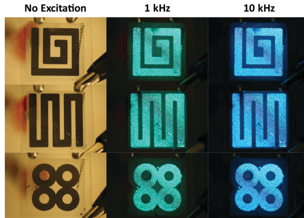
Fig. 4 Demonstration of custom 3D-printed ACEL devices with various geometric patterns under ambient conditions with no excitation, and with a 245 V source under varying excitation frequencies showing visual changes in color.
