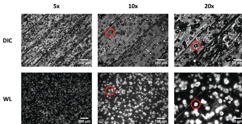
Fig. 2 Differential interference contrast (DIC) and white light (WL) microscopy images for 3D-printed PLA/phosphor thin film samples (20% phosphor in PLA by weight) at increasing levels of magnification. Red circles indicate representative ZnS:Cu phosphor particles embedded in PLA under DIC and WL excitation, respectively. The diagonal lines visible in the images are a result of material deposition and nozzle movement occurring during the 3D printing process and material deposition/sample fabrication.
